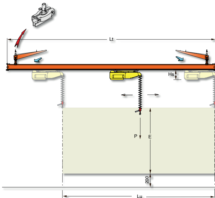
MINIPARTNER overhead trolley mounted "MPS"
